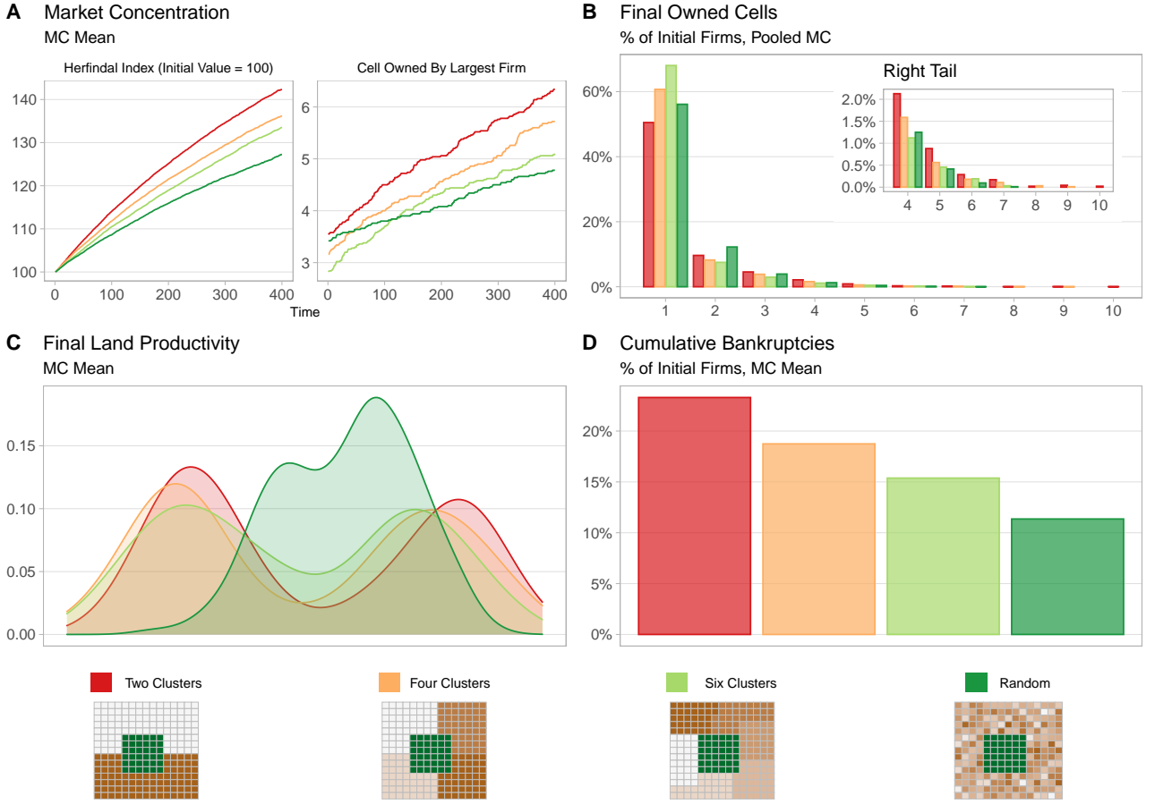
Figure 6: Results for different spatial scenarios of initial land productivity. 50 Monte Carlo replications. See Table D.2 for further details.
