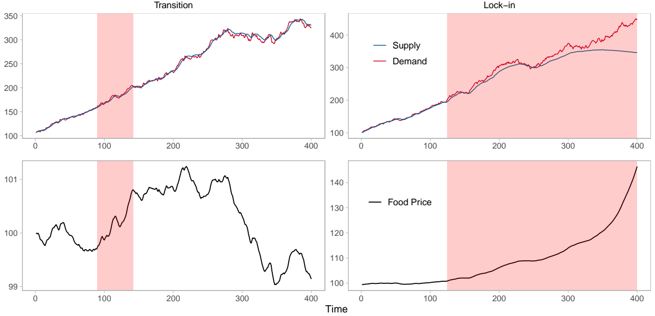
Figure 8: Transition and lock-in scenarios in the model. Two different single runs of the model, exemplifying the main types of dynamics observed in the model: rapid transition to sustainable farming and conventional lock-in. For each run, distance between total demand and supply and food price dynamic are shown. Red areas correspond to periods of insufficient food supply.
